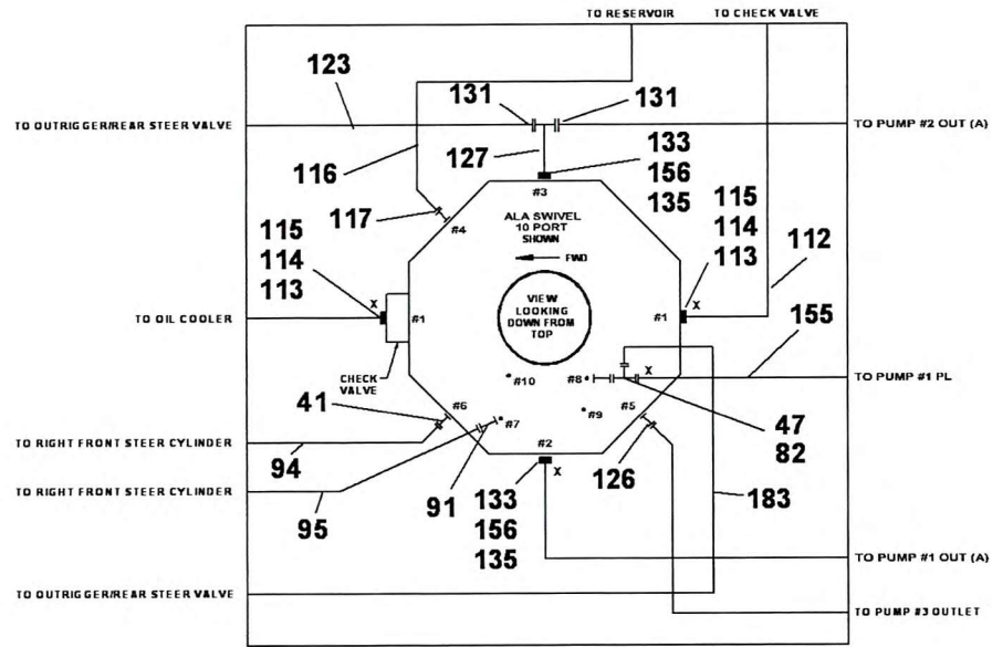
SWIVEL PLUMBING FOR ALA SWIVEL
