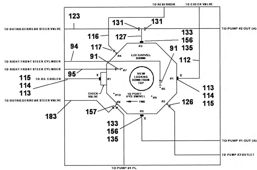
SWIVEL PLUMBING FOR LDI SWIVEL
