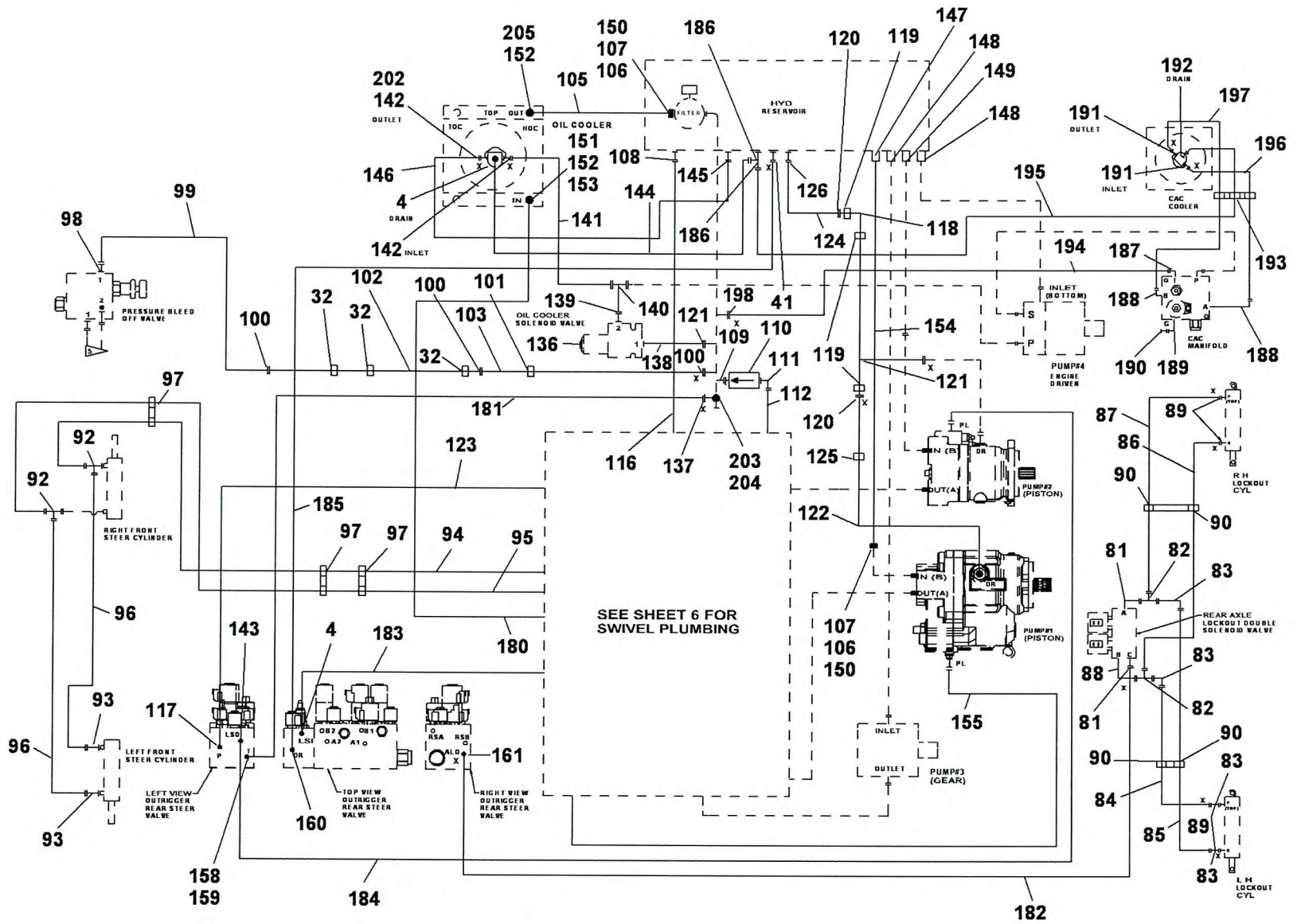
SUPPLY,PRESSURE & RETURN FRONT STEER AND REAR AXLE L/O
